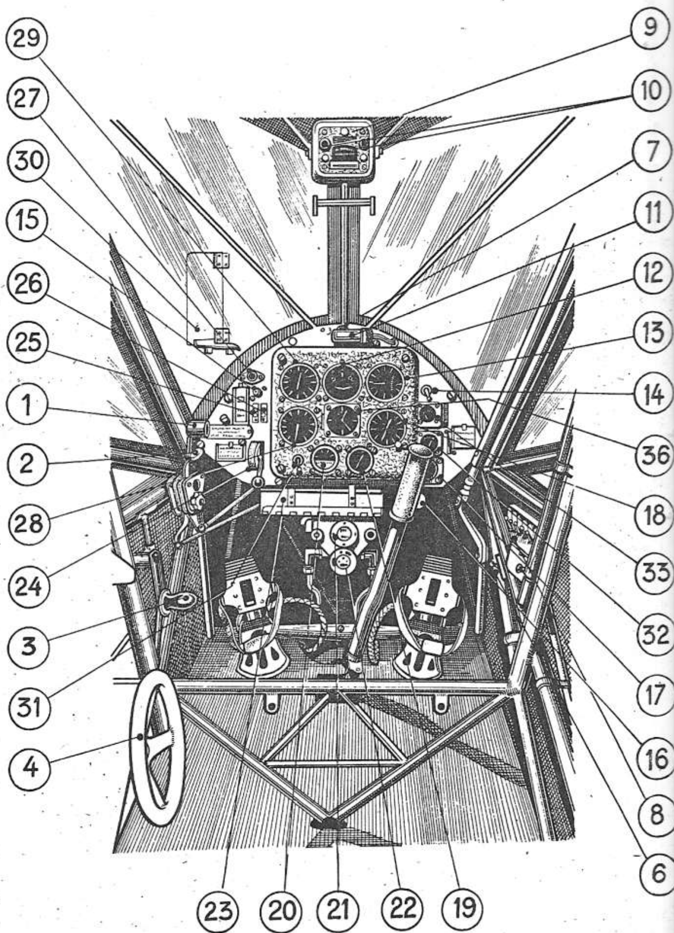
Fig.22 B _ Cabine avion Criket II B
